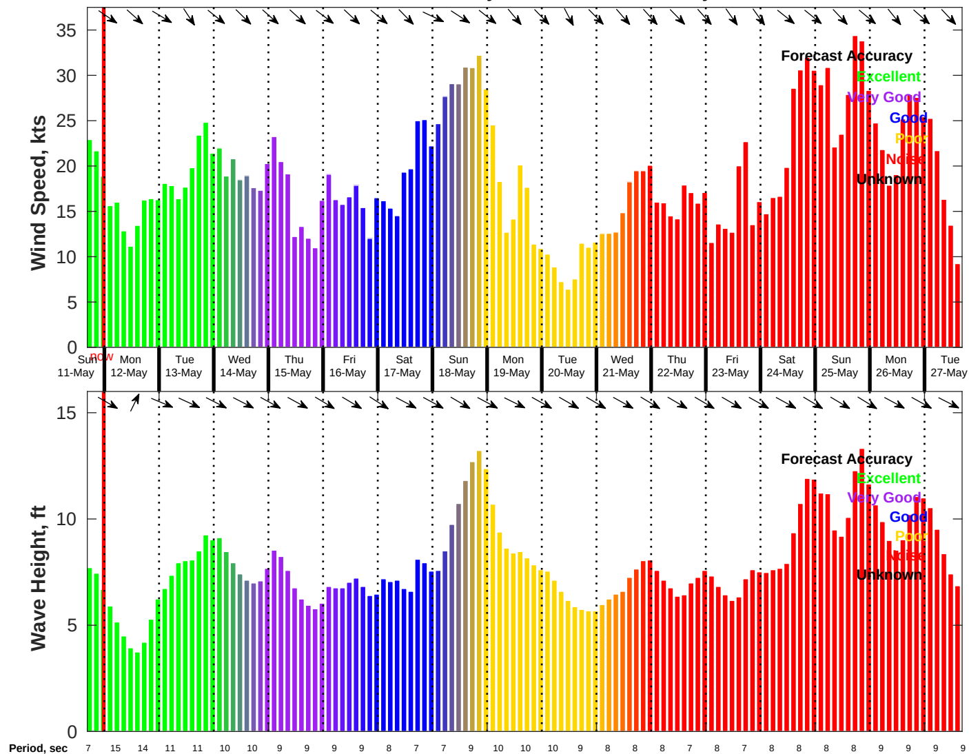
Wind & Wave Forecast for NDBC 46011 from 11-May-2025 16:00:00 to 27-May-2025 16:00:00
