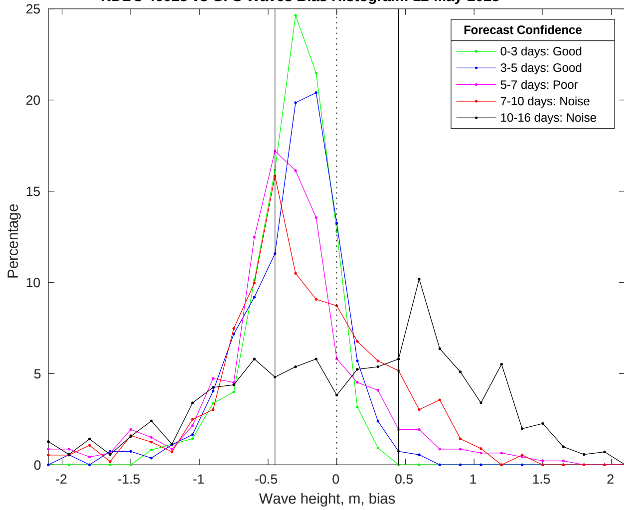
NDBC 46028 vs GFS Waves Bias Histogram: 12-May-2025
