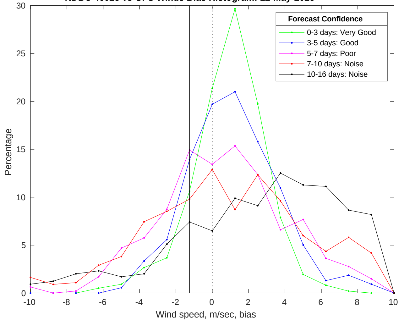
NDBC 46028 vs GFS Winds Bias Histogram: 12-May-2025
