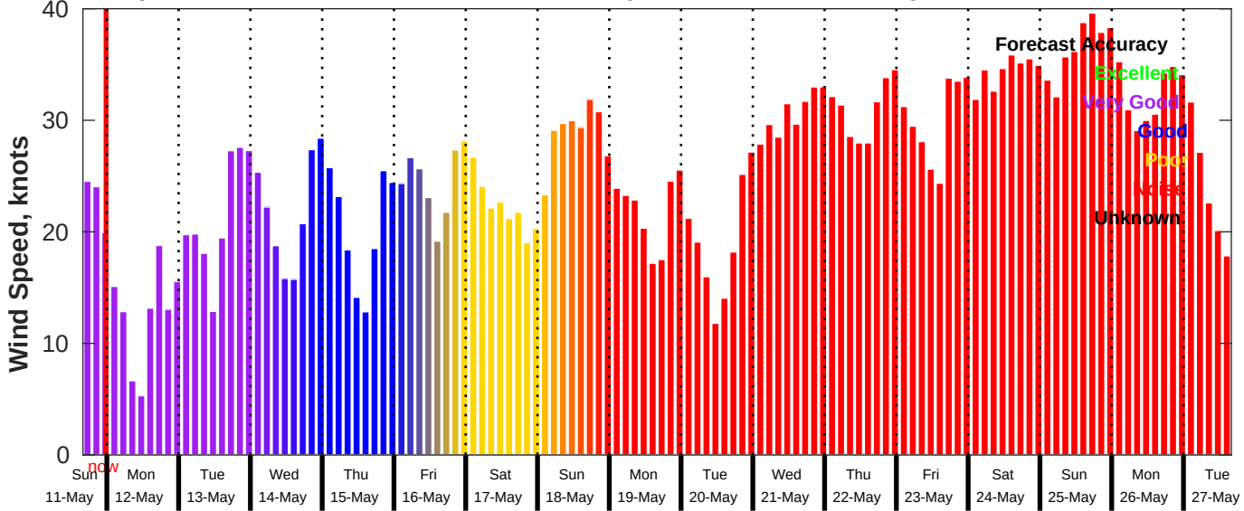
GFS Wind Speed Forecast for NDBC 46028 from 11-May-2025 16:00:00 to 27-May-2025 16:00:00
