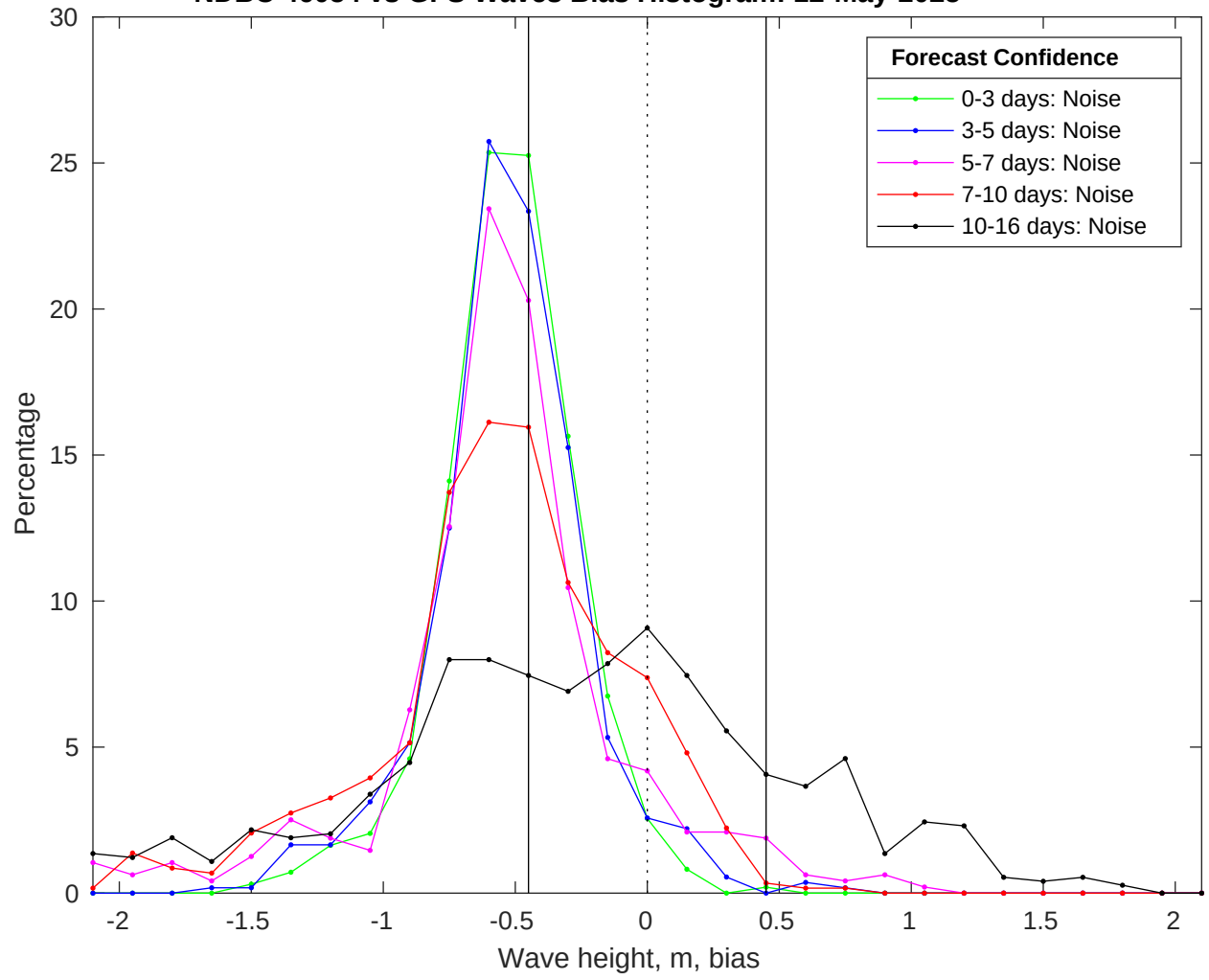
NDBC 46054 vs GFS Waves Bias Histogram: 12-May-2025
