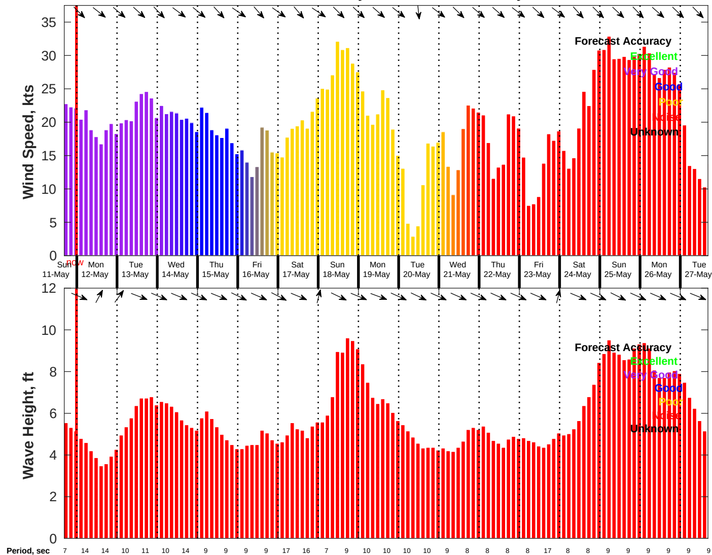
Wind & Wave Forecast for NDBC 46054 from 11-May-2025 16:00:00 to 27-May-2025 16:00:00
