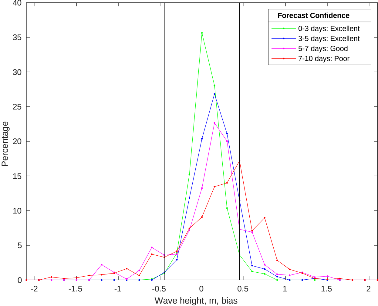
NDBC 46069 vs CMEMS Waves Bias Histogram: 12-May-2025
