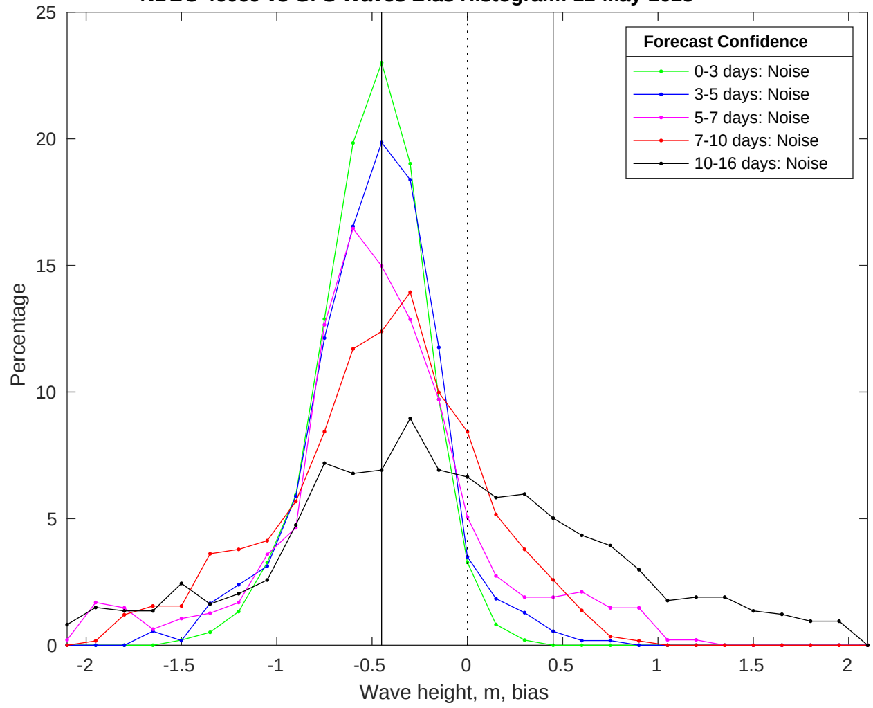
NDBC 46069 vs GFS Waves Bias Histogram: 12-May-2025
