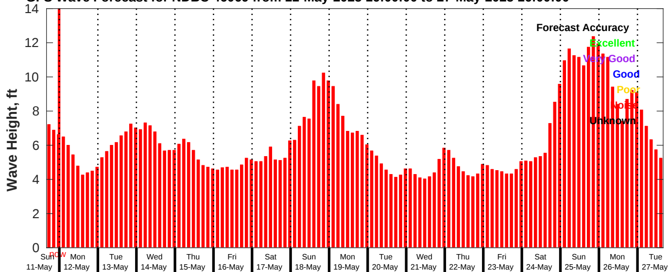
GFS Wave Forecast for NDBC 46069 from 11-May-2025 16:00:00 to 27-May-2025 16:00:00
