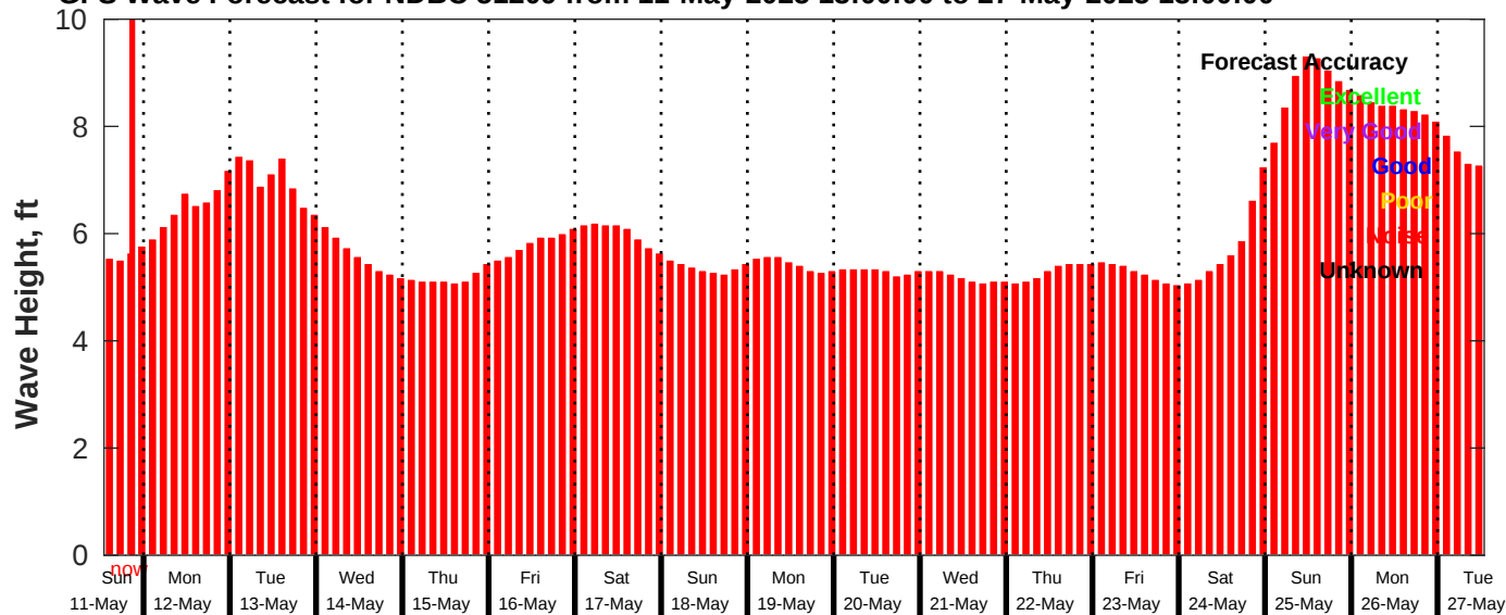
GFS Wave Forecast for NDBC 51209 from 11-May-2025 13:00:00 to 27-May-2025 13:00:00
