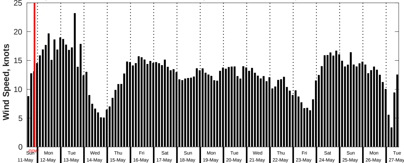
GFS Wind Speed Forecast for NDBC 51209 from 11-May-2025 13:00:00 to 27-May-2025 13:00:00
