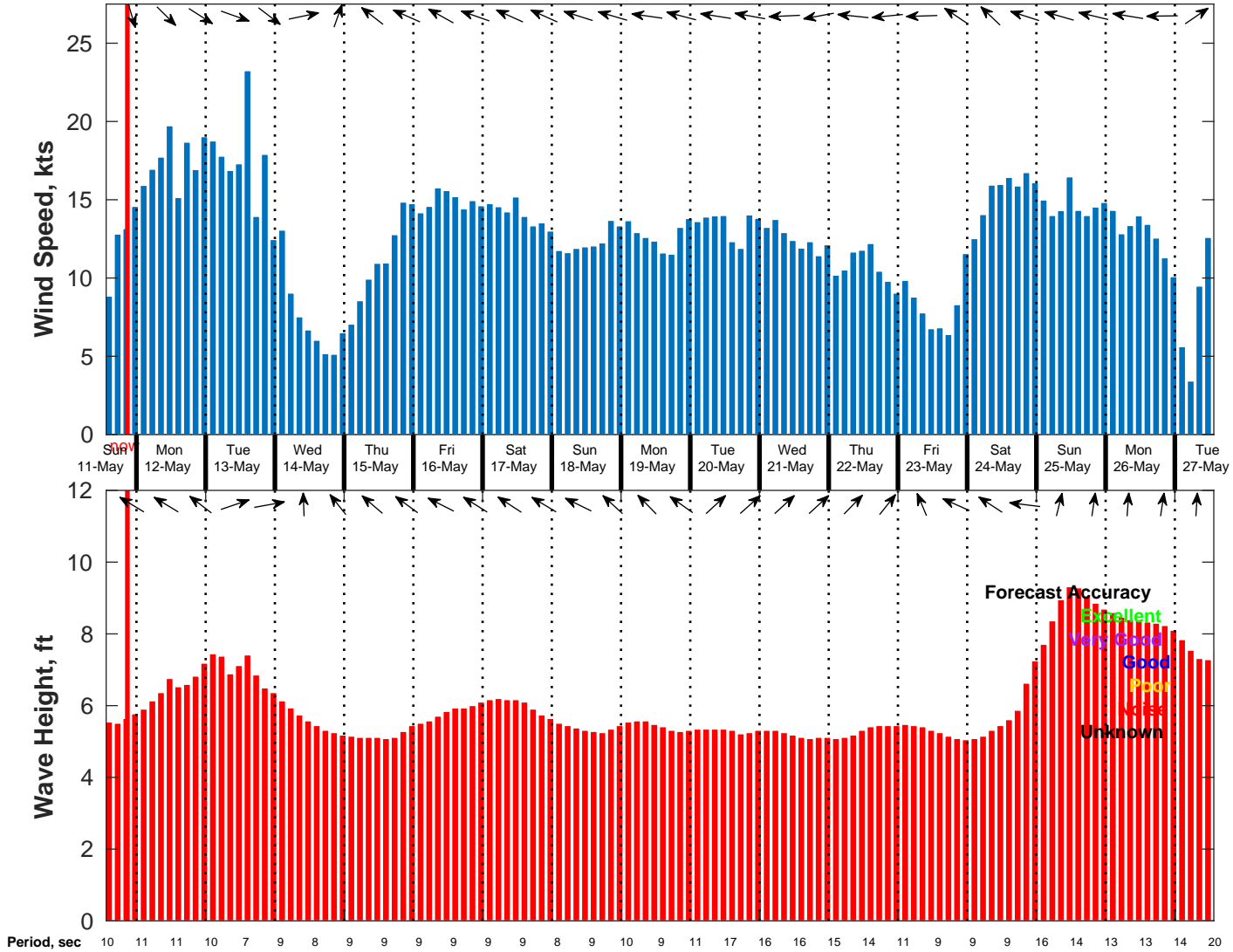
Wind & Wave Forecast for NDBC 51209 from 11-May-2025 13:00:00 to 27-May-2025 13:00:00
