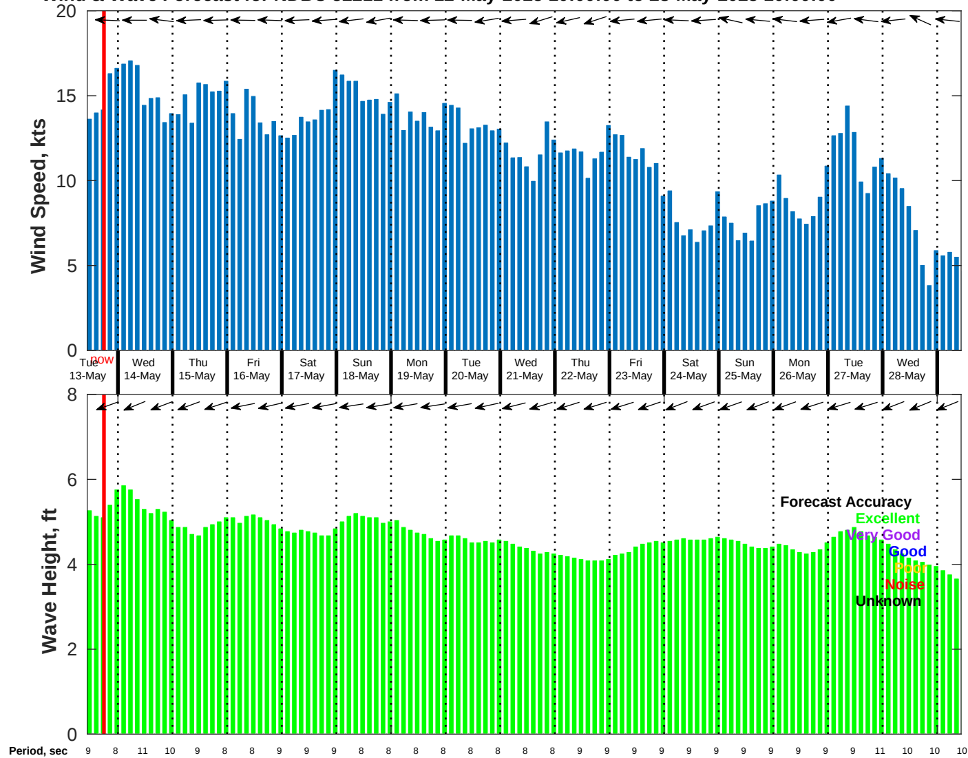
Wind & Wave Forecast for NDBC 52211 from 12-May-2025 10:00:00 to 28-May-2025 10:00:00
