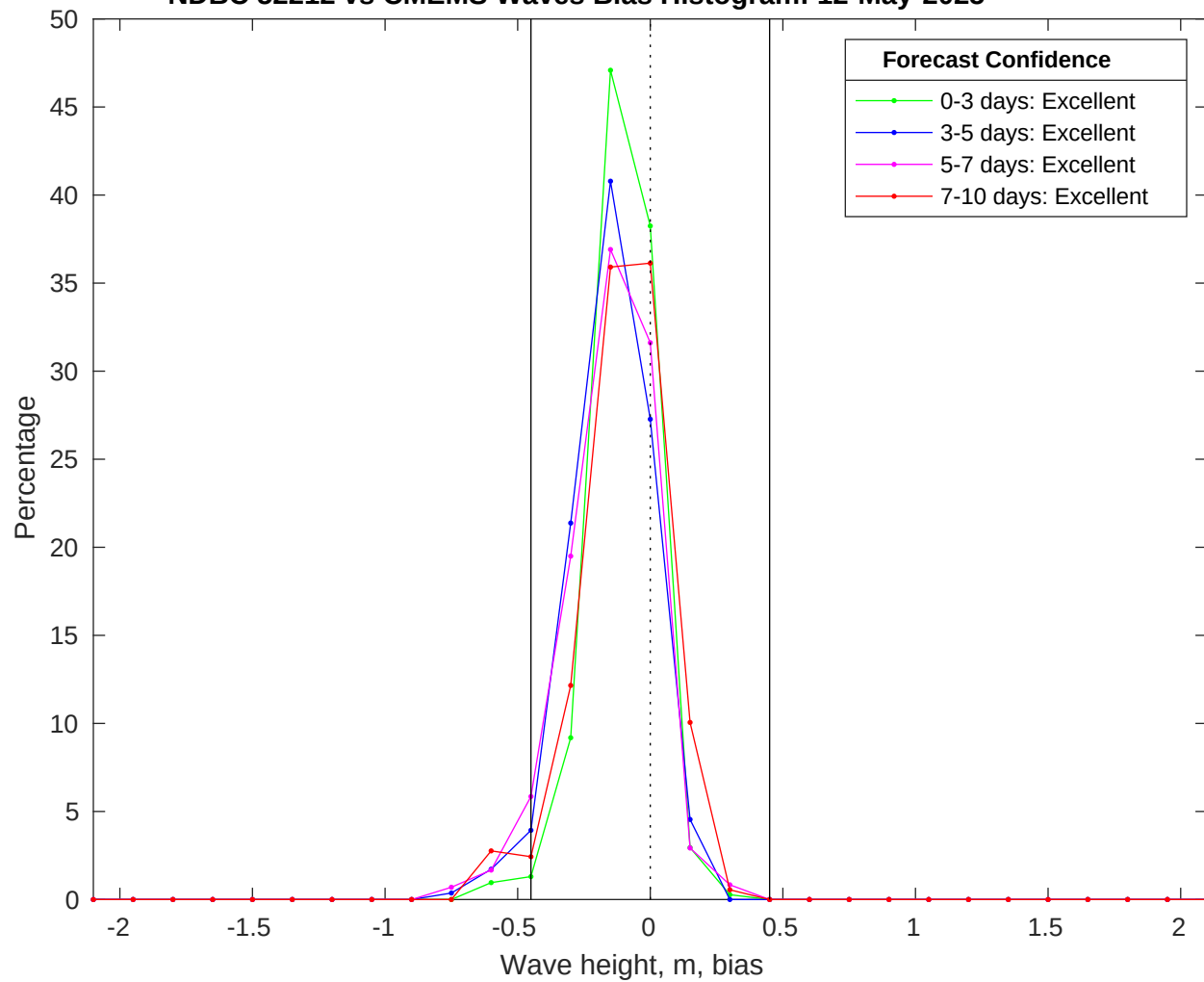
NDBC 52212 vs CMEMS Waves Bias Histogram: 12-May-2025
