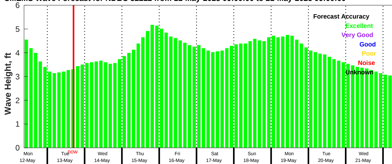
CMEMS Wave Forecast for NDBC 52212 from 11-May-2025 09:00:00 to 21-May-2025 09:00:00
