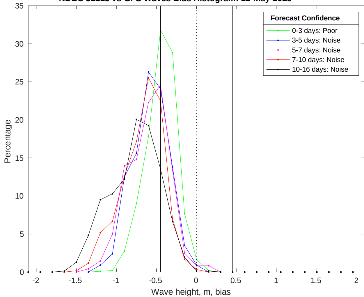
NDBC 52213 vs GFS Waves Bias Histogram: 12-May-2025
