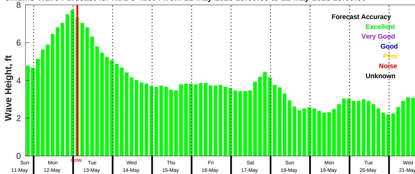
CMEMS Wave Forecast for NDBC 41004 from 11-May-2025 19:00:00 to 21-May-2025 19:00:00
