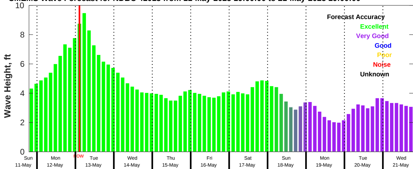
CMEMS Wave Forecast for NDBC 41013 from 11-May-2025 19:00:00 to 21-May-2025 19:00:00
