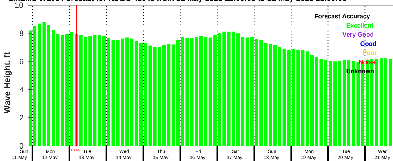
CMEMS Wave Forecast for NDBC 41040 from 11-May-2025 21:00:00 to 21-May-2025 21:00:00
