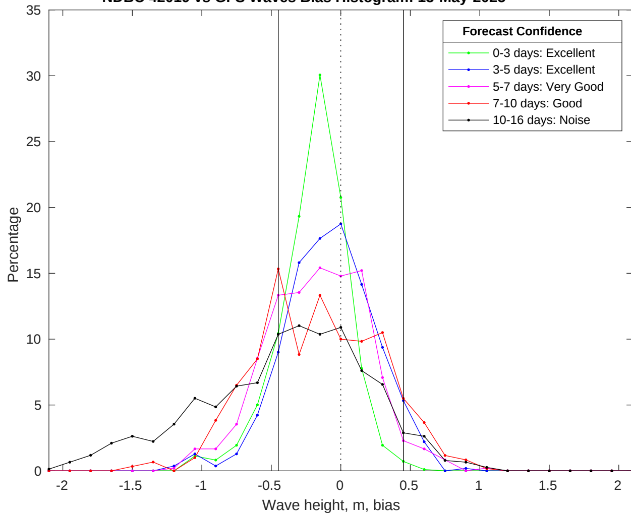
NDBC 42019 vs GFS Waves Bias Histogram: 13-May-2025
