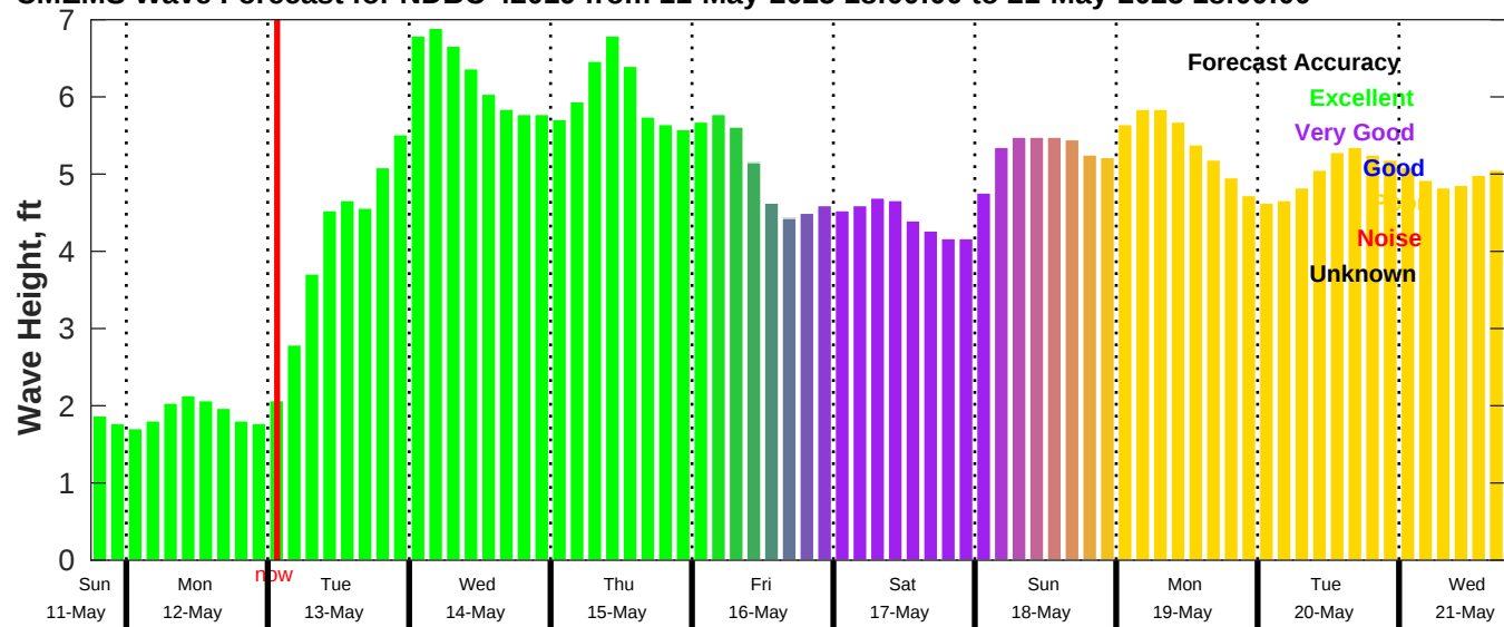
CMEMS Wave Forecast for NDBC 42019 from 11-May-2025 18:00:00 to 21-May-2025 18:00:00
