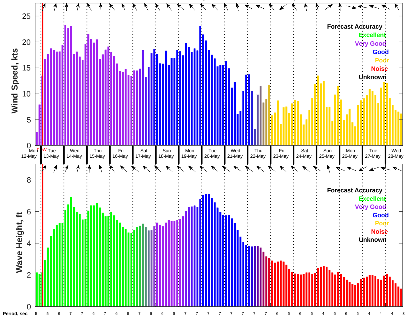
Wind & Wave Forecast for NDBC 42019 from 12-May-2025 18:00:00 to 28-May-2025 18:00:00
