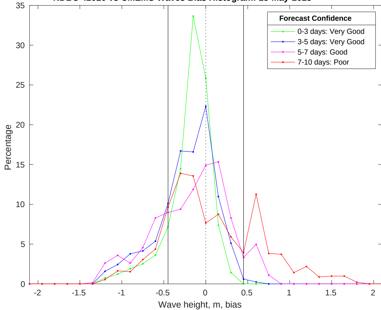
NDBC 42020 vs CMEMS Waves Bias Histogram: 13-May-2025
