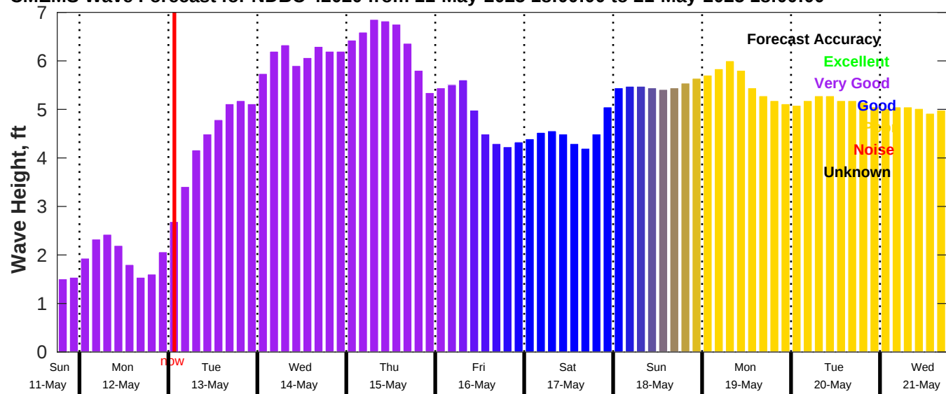
CMEMS Wave Forecast for NDBC 42020 from 11-May-2025 18:00:00 to 21-May-2025 18:00:00
