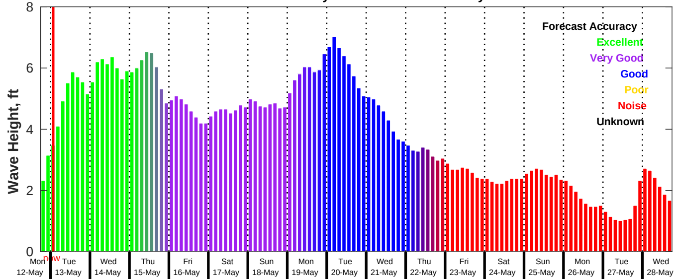
GFS Wave Forecast for NDBC 42020 from 12-May-2025 18:00:00 to 28-May-2025 18:00:00
