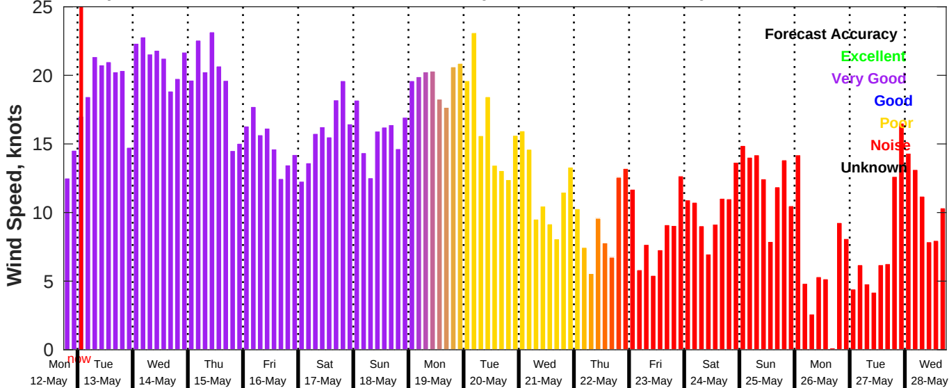
GFS Wind Speed Forecast for NDBC 42020 from 12-May-2025 18:00:00 to 28-May-2025 18:00:00
