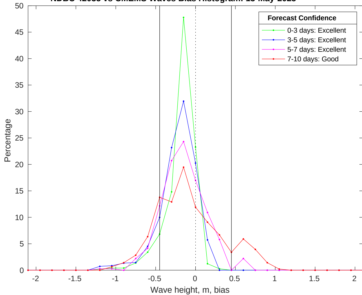
NDBC 42035 vs CMEMS Waves Bias Histogram: 13-May-2025
