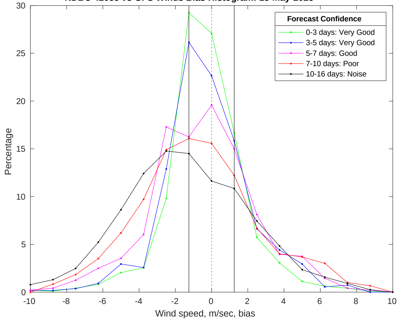
NDBC 42035 vs GFS Winds Bias Histogram: 13-May-2025
