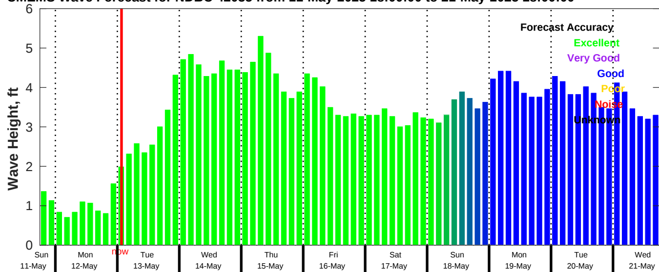
CMEMS Wave Forecast for NDBC 42035 from 11-May-2025 18:00:00 to 21-May-2025 18:00:00
