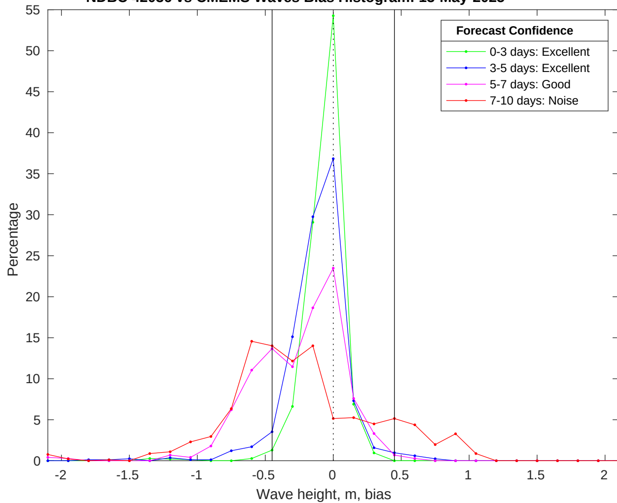
NDBC 42036 vs CMEMS Waves Bias Histogram: 13-May-2025
