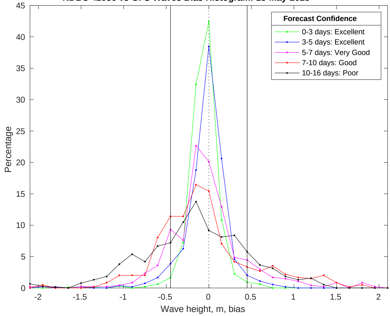
NDBC 42036 vs GFS Waves Bias Histogram: 13-May-2025
