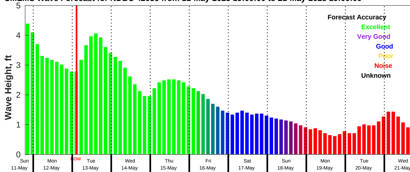
CMEMS Wave Forecast for NDBC 42036 from 11-May-2025 19:00:00 to 21-May-2025 19:00:00
