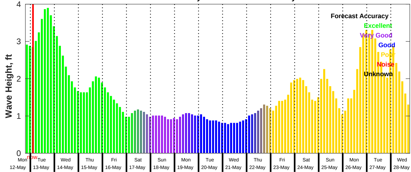
GFS Wave Forecast for NDBC 42036 from 12-May-2025 19:00:00 to 28-May-2025 19:00:00
