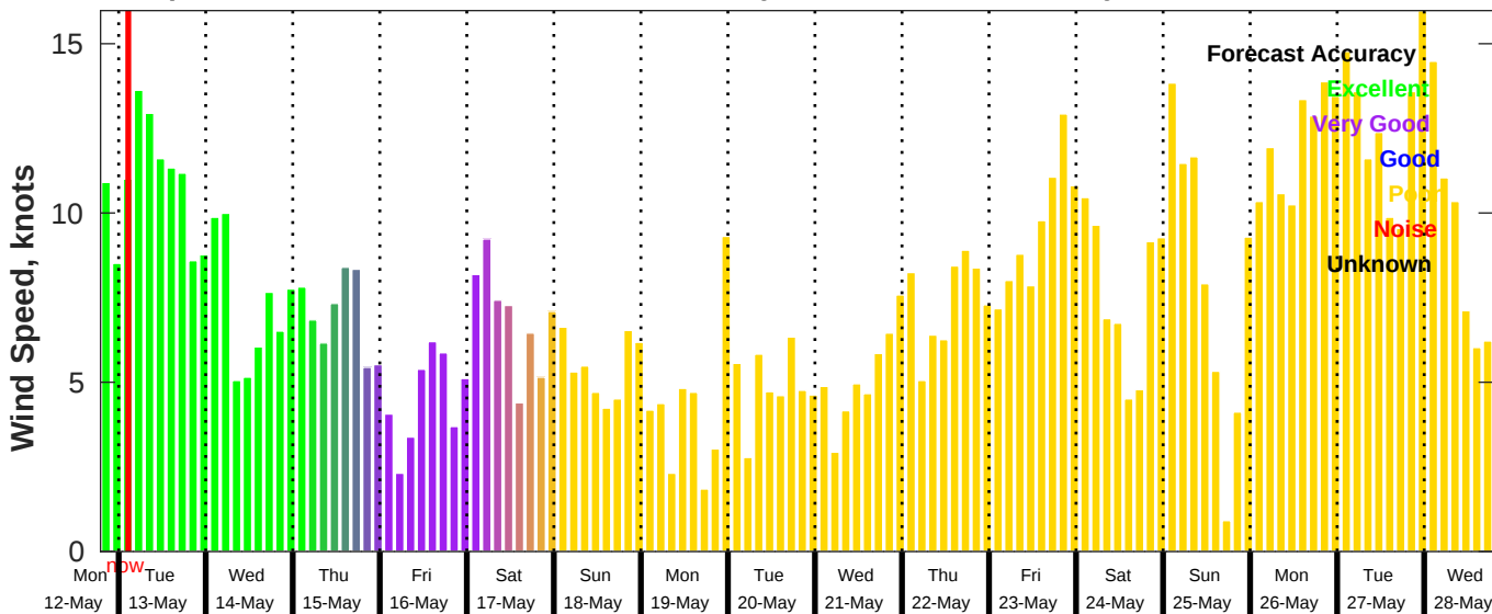
GFS Wind Speed Forecast for NDBC 42036 from 12-May-2025 19:00:00 to 28-May-2025 19:00:00
