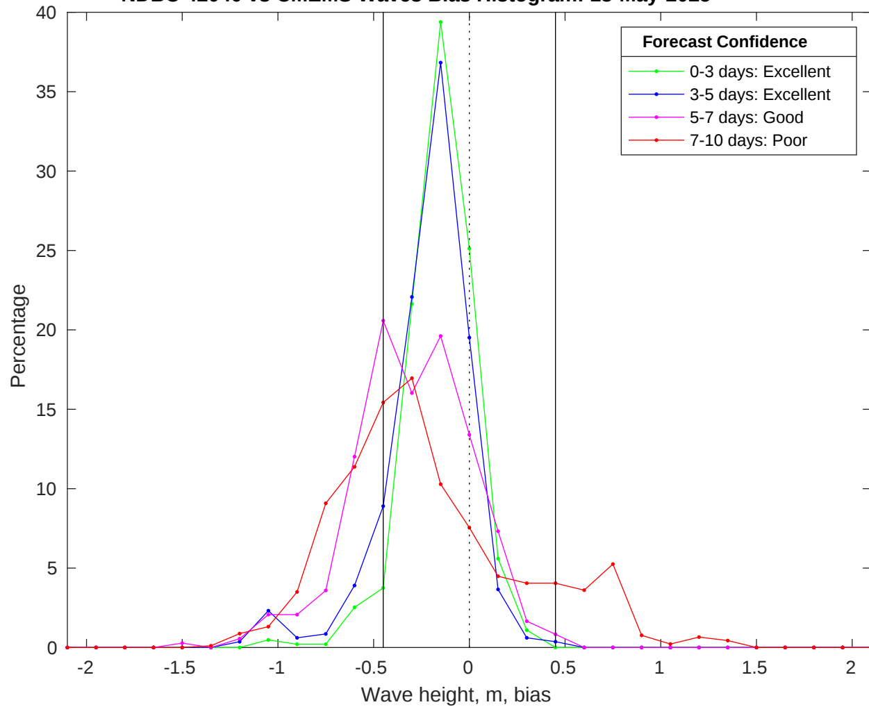
NDBC 42040 vs CMEMS Waves Bias Histogram: 13-May-2025
