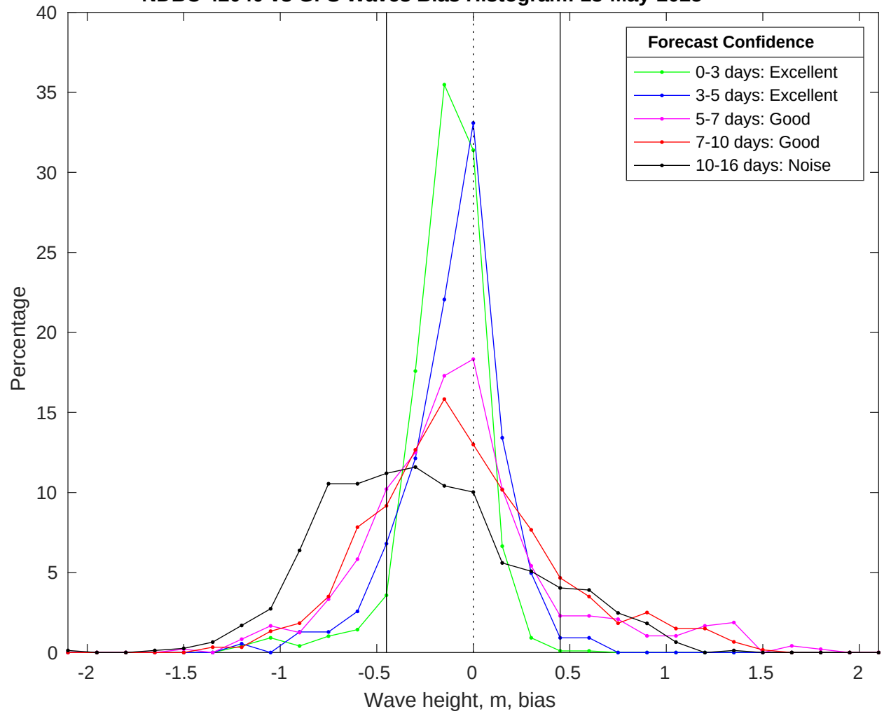
NDBC 42040 vs GFS Waves Bias Histogram: 13-May-2025
