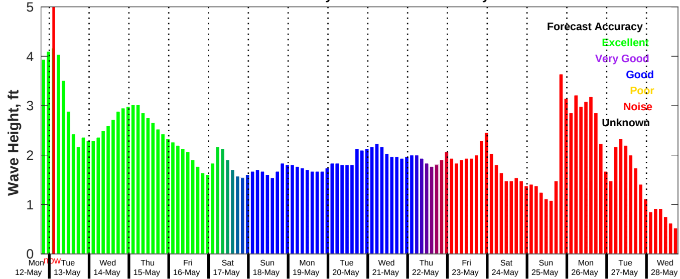
GFS Wave Forecast for NDBC 42040 from 12-May-2025 19:00:00 to 28-May-2025 19:00:00
