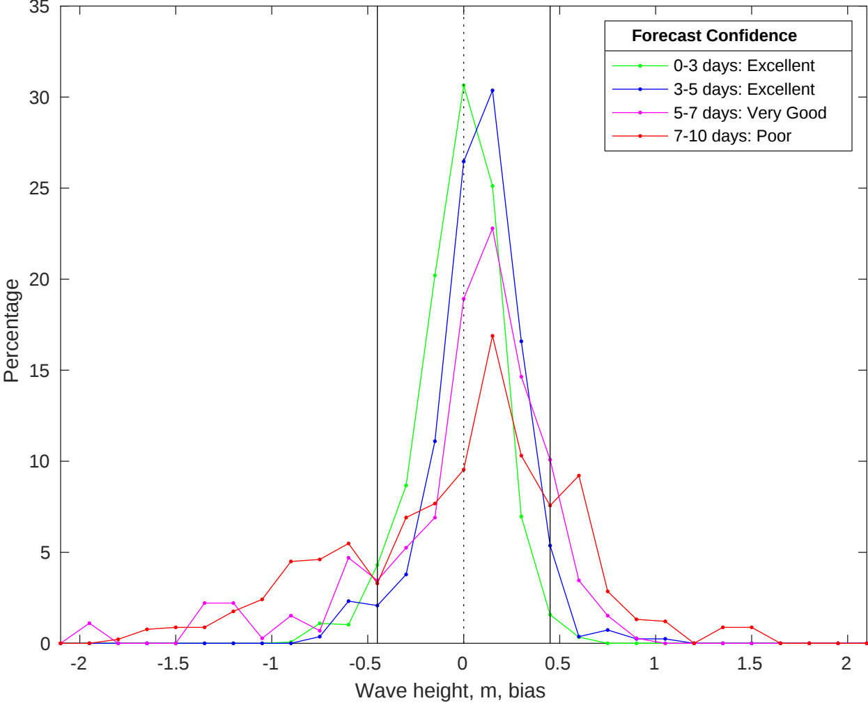
NDBC 46011 vs CMEMS Waves Bias Histogram: 13-May-2025
