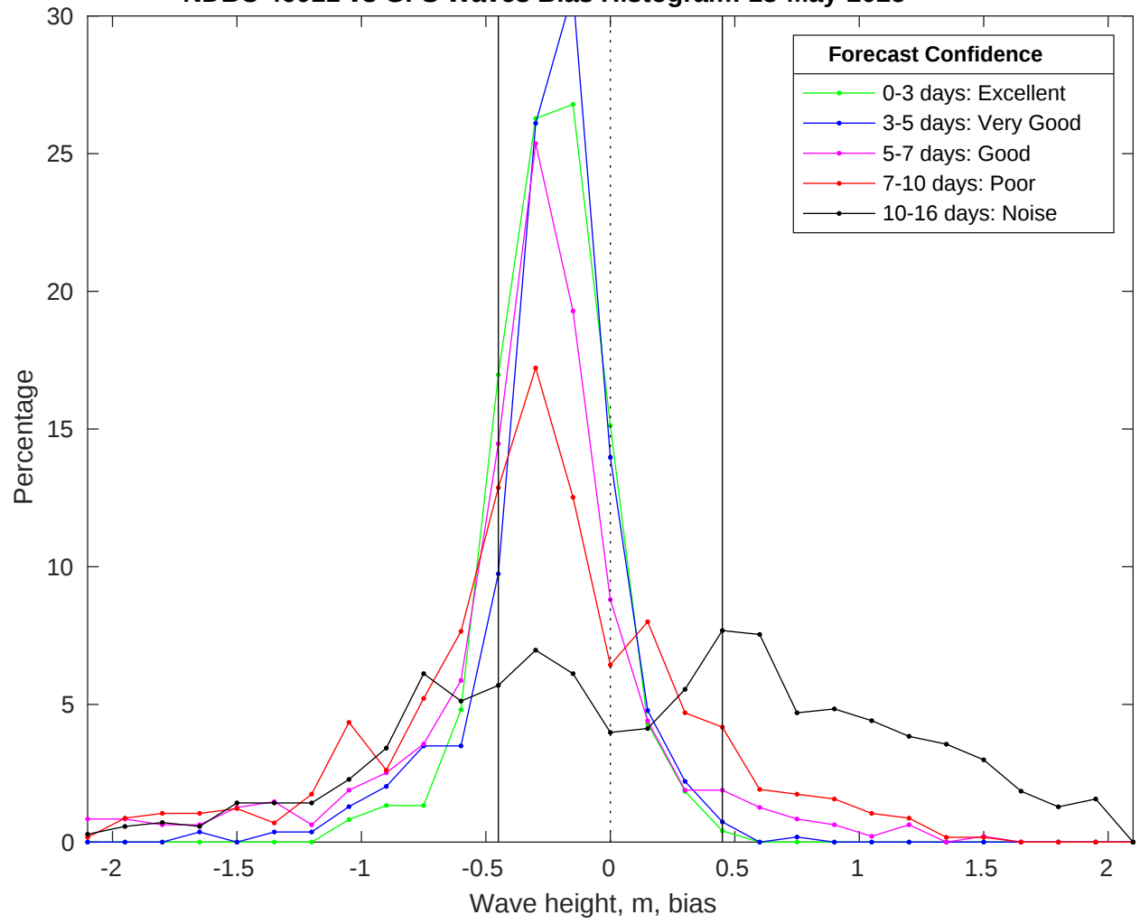
NDBC 46011 vs GFS Waves Bias Histogram: 13-May-2025
