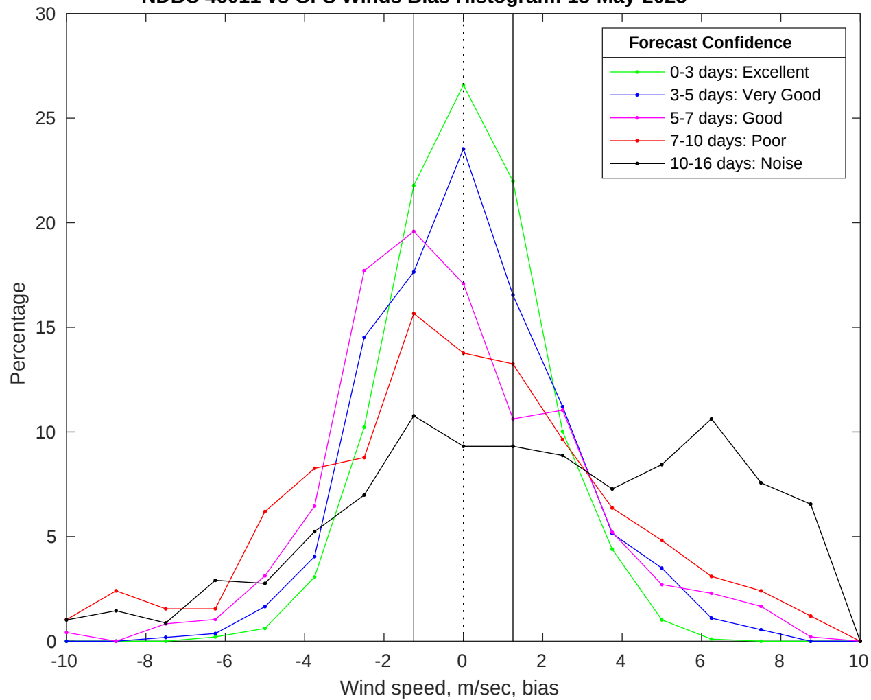
NDBC 46011 vs GFS Winds Bias Histogram: 13-May-2025
