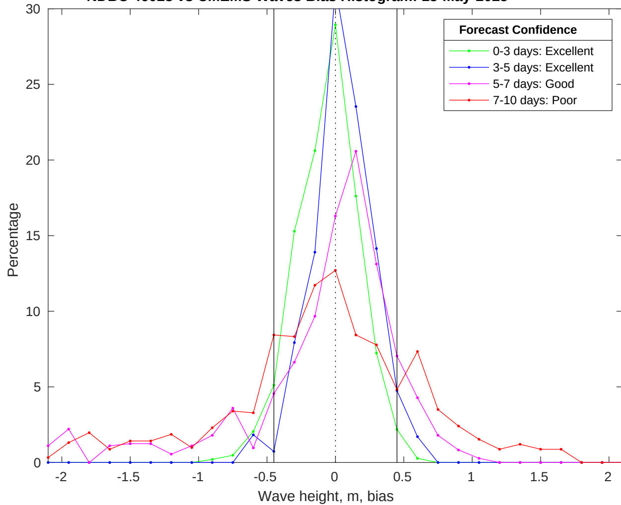
NDBC 46028 vs CMEMS Waves Bias Histogram: 13-May-2025
