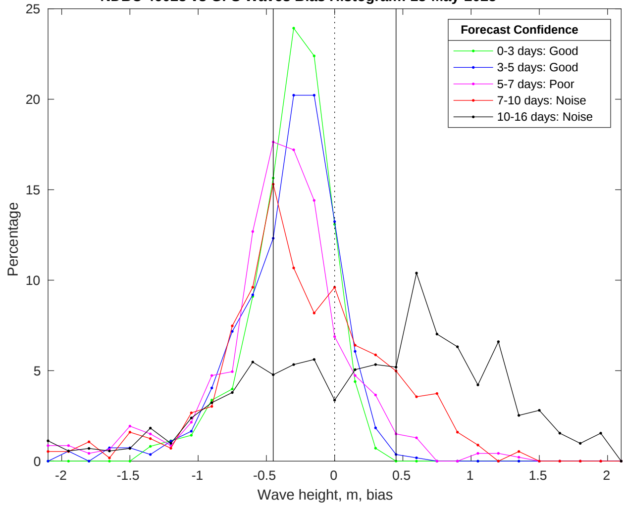
NDBC 46028 vs GFS Waves Bias Histogram: 13-May-2025
