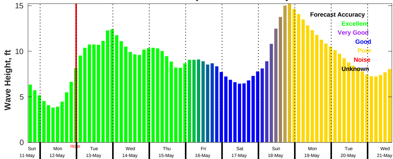
CMEMS Wave Forecast for NDBC 46028 from 11-May-2025 16:00:00 to 21-May-2025 16:00:00
