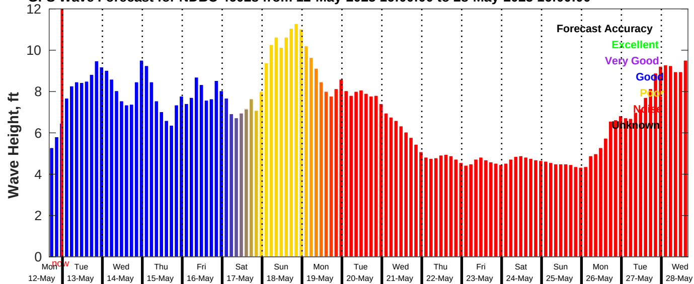
GFS Wave Forecast for NDBC 46028 from 12-May-2025 16:00:00 to 28-May-2025 16:00:00
