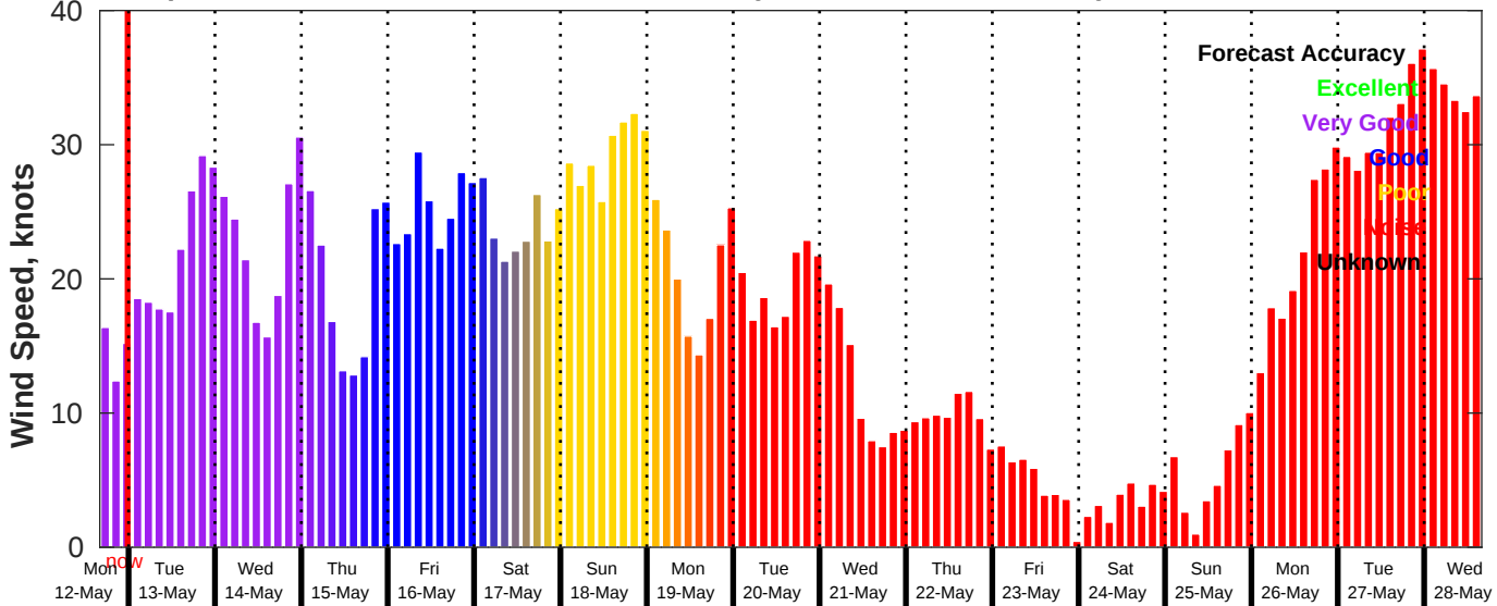
GFS Wind Speed Forecast for NDBC 46028 from 12-May-2025 16:00:00 to 28-May-2025 16:00:00
