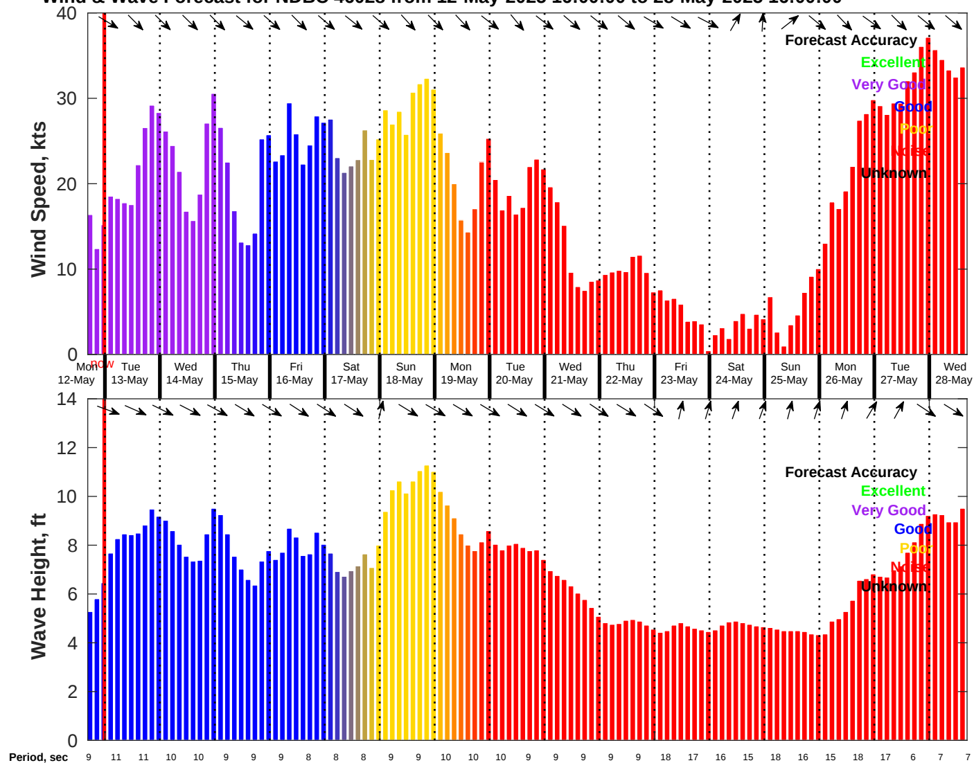
Wind & Wave Forecast for NDBC 46028 from 12-May-2025 16:00:00 to 28-May-2025 16:00:00
