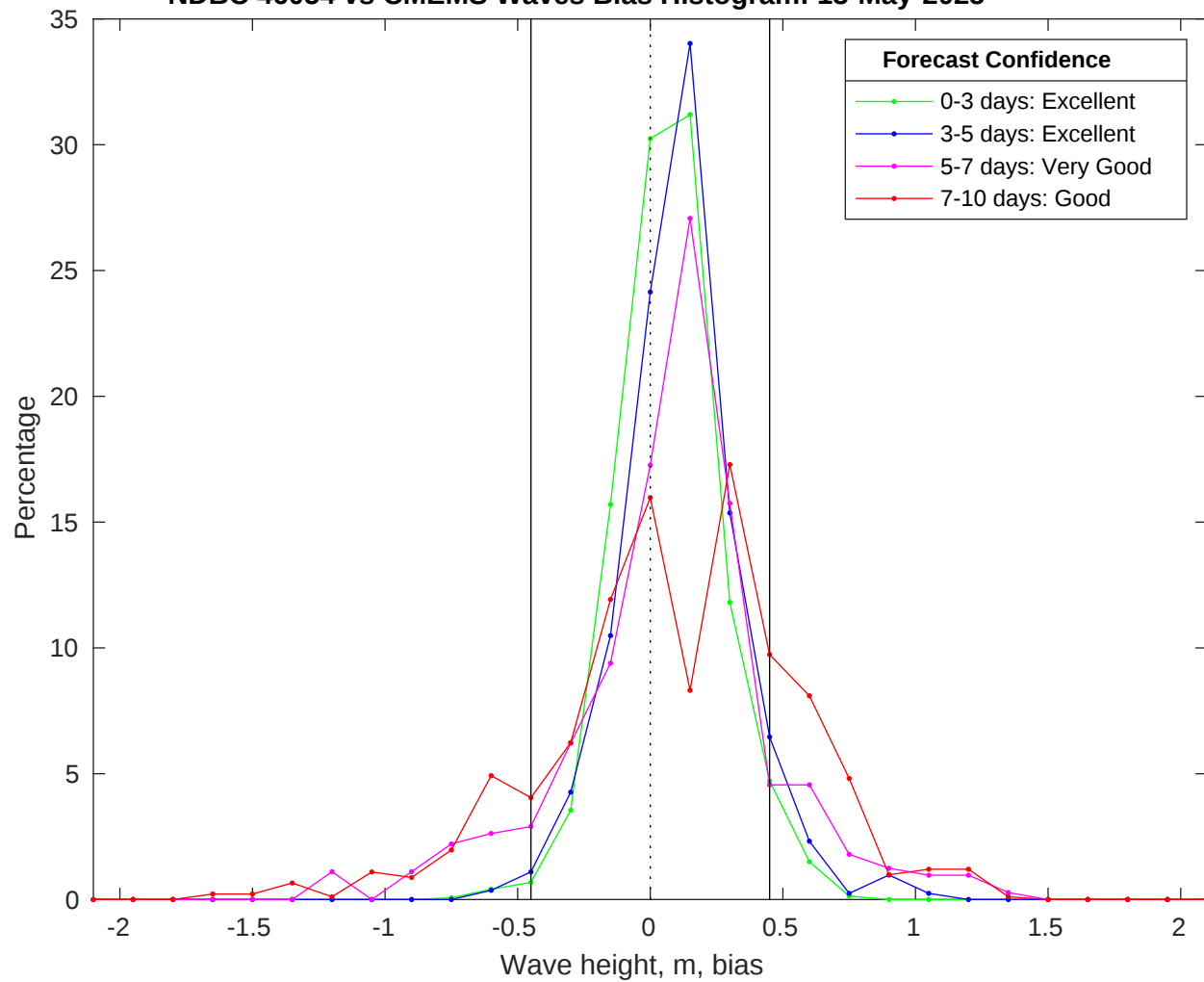
NDBC 46054 vs CMEMS Waves Bias Histogram: 13-May-2025
