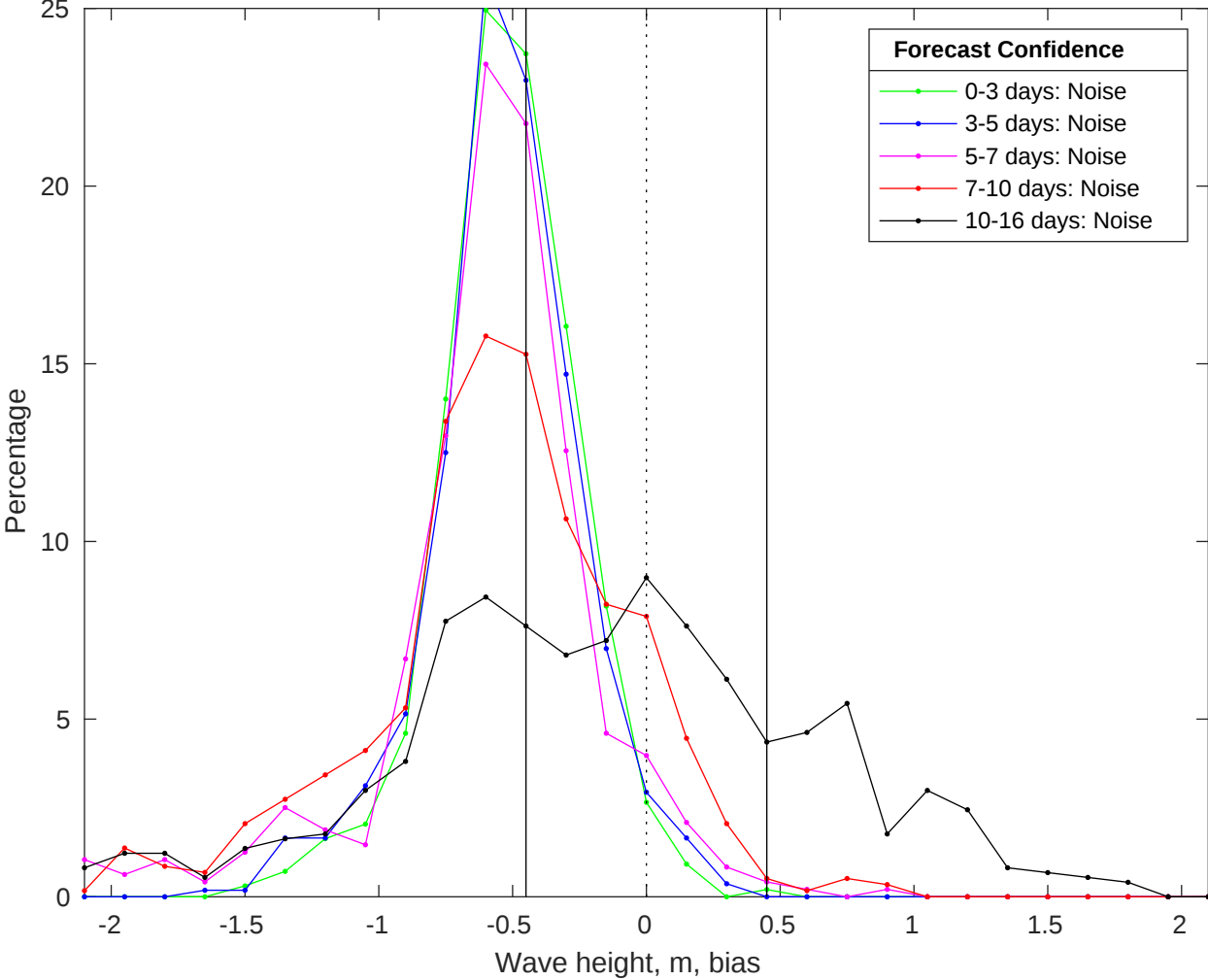
NDBC 46054 vs GFS Waves Bias Histogram: 13-May-2025
