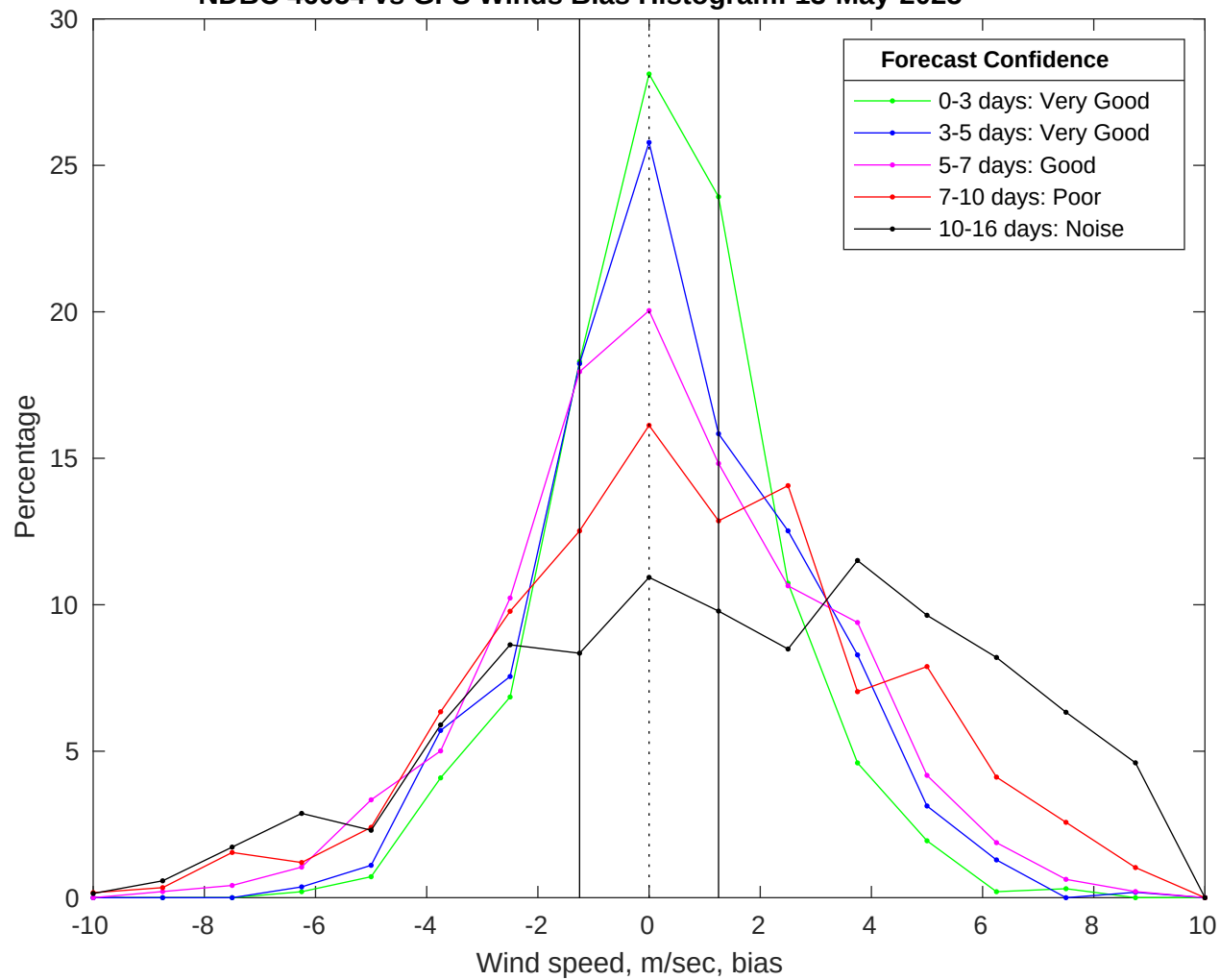
NDBC 46054 vs GFS Winds Bias Histogram: 13-May-2025
