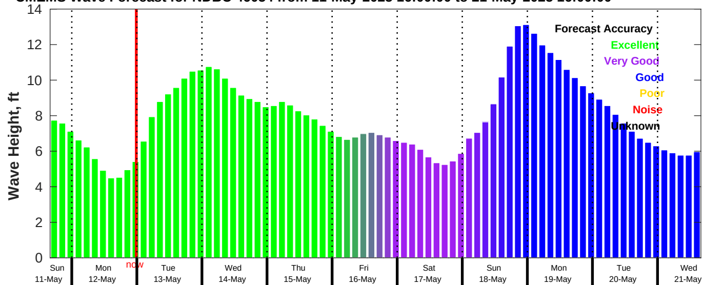
CMEMS Wave Forecast for NDBC 46054 from 11-May-2025 16:00:00 to 21-May-2025 16:00:00
